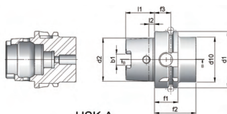
HSK A
